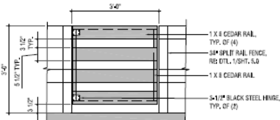
2 36" SPLIT RAIL GATE SCALE: 3/4" = 1'-0"
