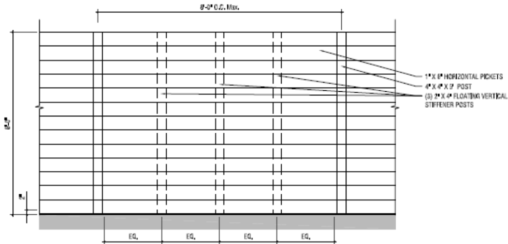
3 6' PRIVACY FENCE SCALE: 3/4" = 1'-0"
